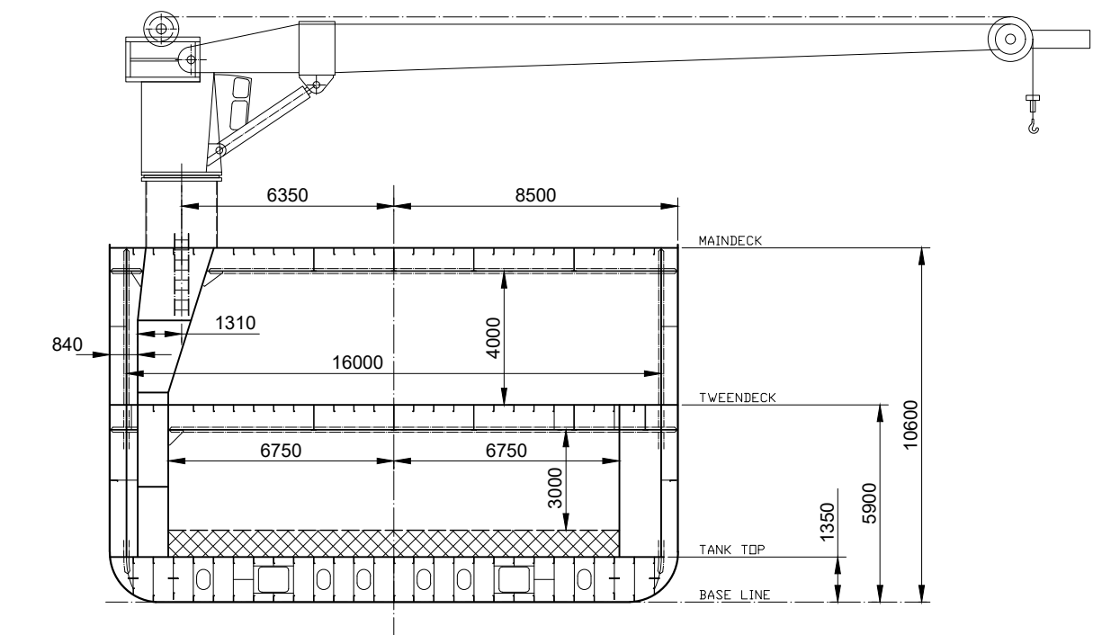
TR.V SECTION - MIDSHIP.
