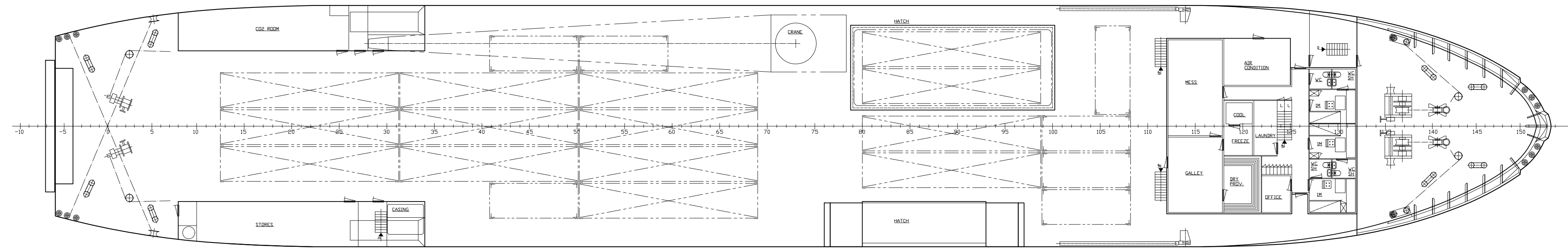
SHELTER DECK
