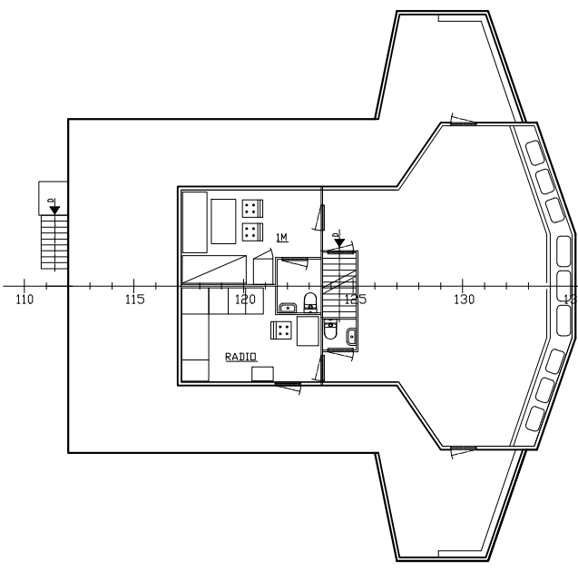
3. BRIDGE DECK
