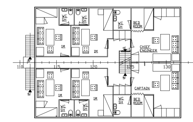
2. BRIDGE DECK
