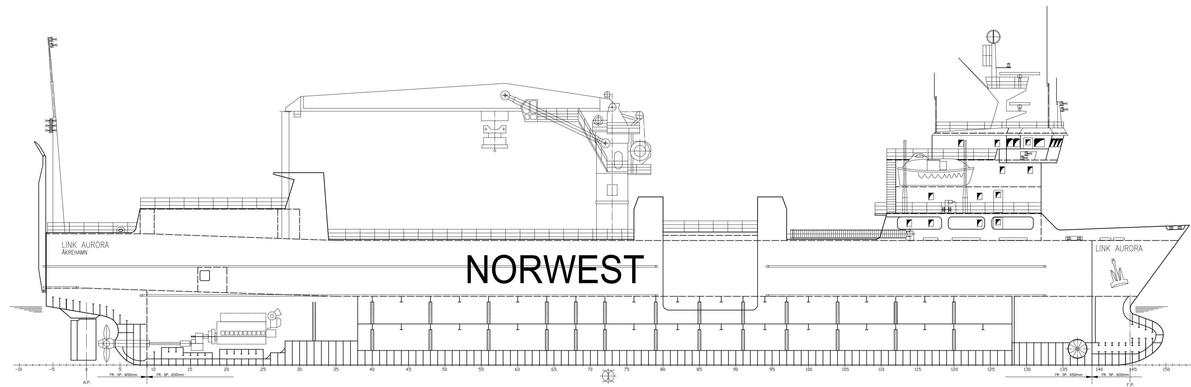
PROFILE
