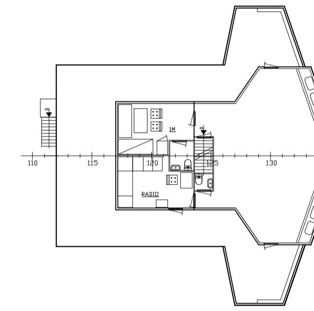
3. BRIDGE DECK
