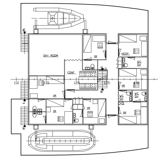
1. BRIDGE DECK
